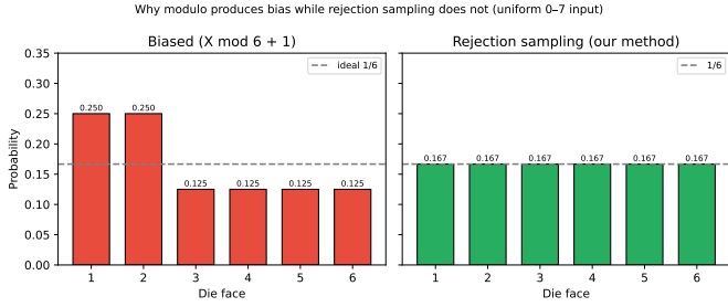
Fig. 1. Comparison of the biased modulo mapping with the exactly uniform distribution obtained by rejection sampling. Both start from a uniform random variable on \{0, \dots, 7\} .
