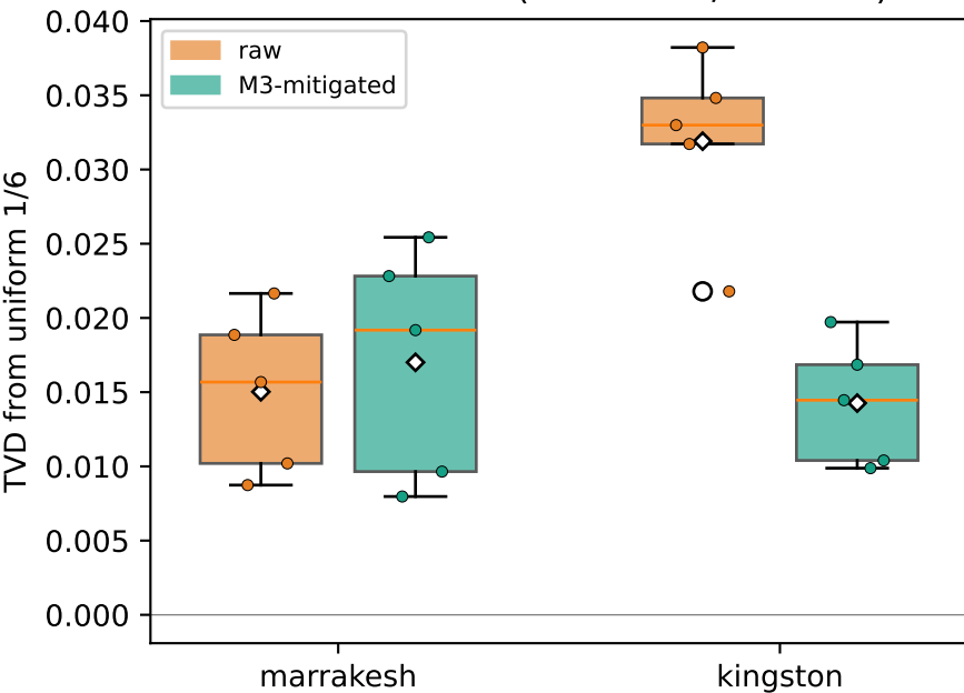
Run-to-run TVD ( N = 5 runs/backend)
