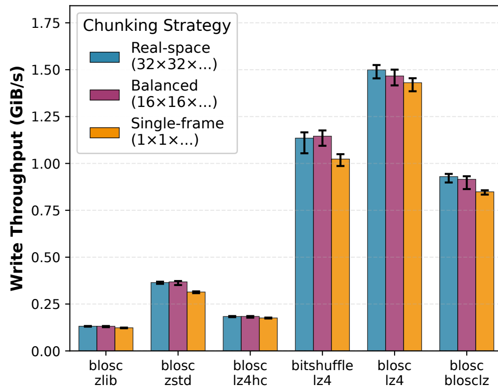
B) Write Throughput
