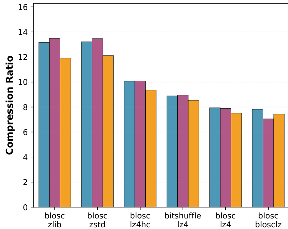
A) Compression Performance
