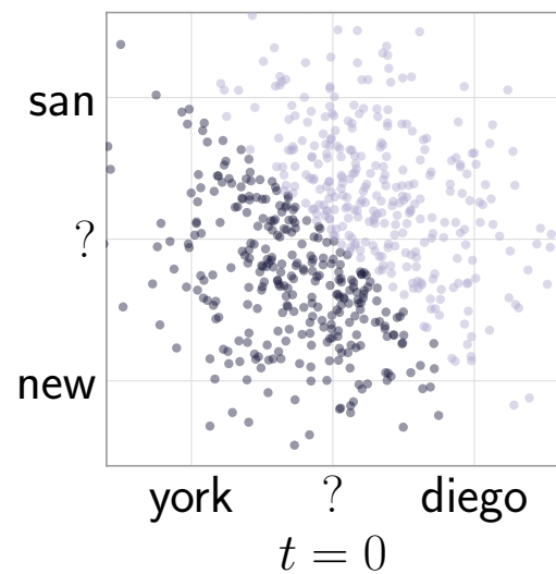
Continuous Flow (Ours)
