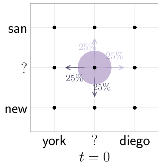
Masked Discrete Diffusion
