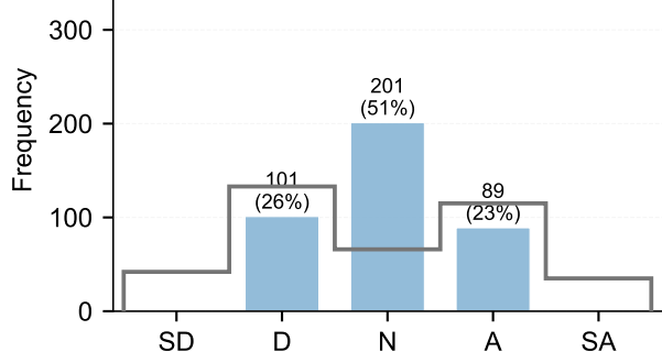
GPT-5-Mini
