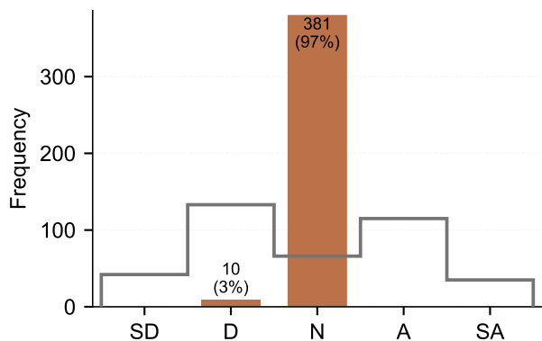
Gemini-3-Flash-Preview
