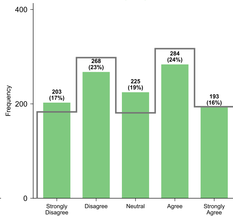
Olmo-3.1-32B-Instruct (DPO)
