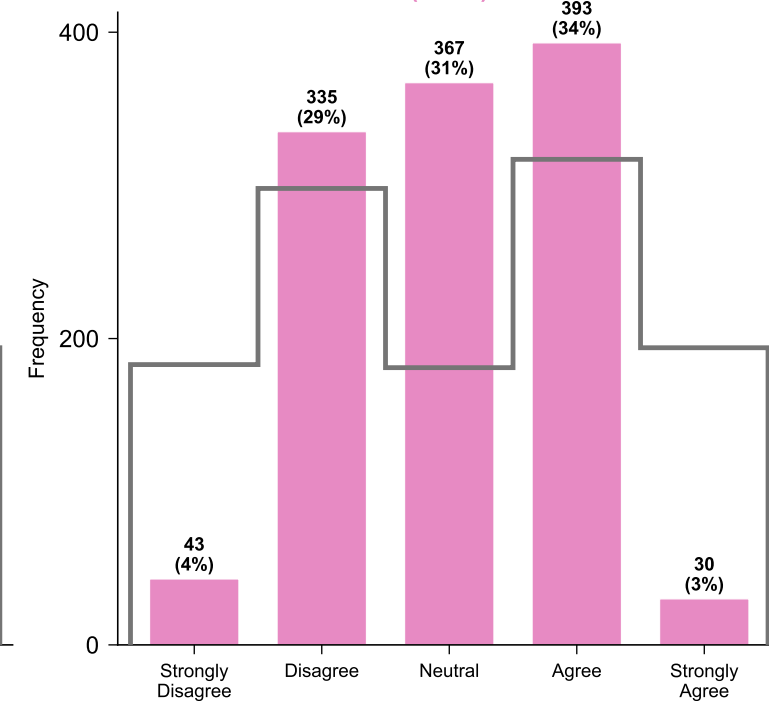
Olmo-3.1-32B-Instruct (Final)
