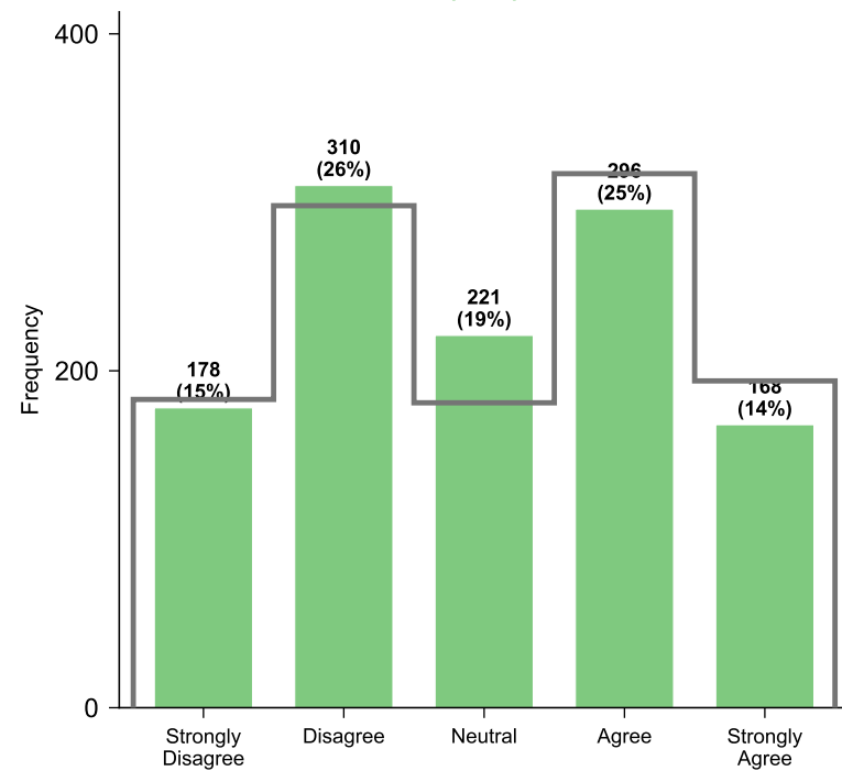
Olmo-3.1-32B-Instruct (SFT)
