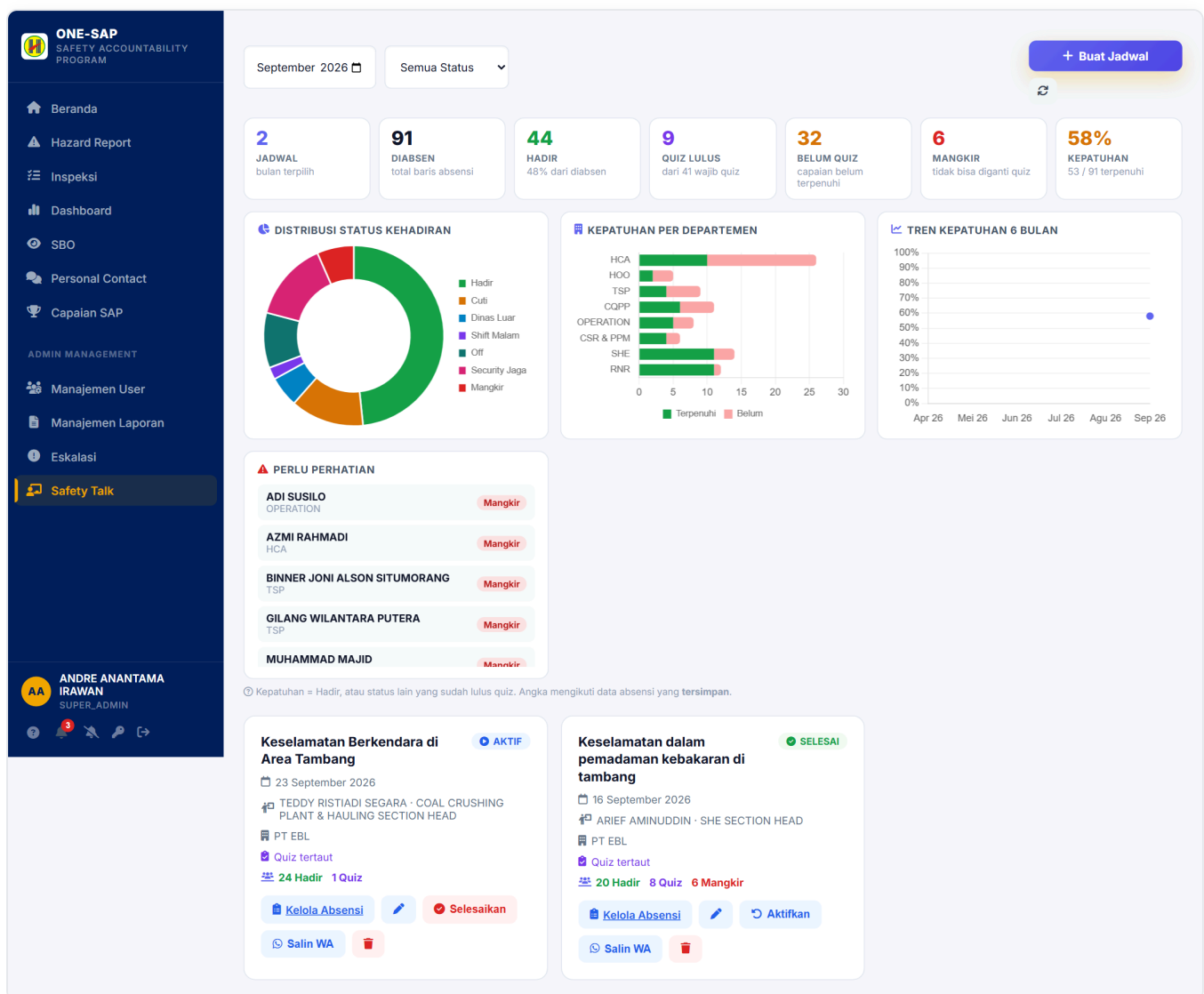
Gambar 13.1 Daftar Jadwal Safety Talk
