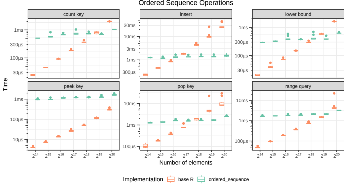
Figure 3: Benchmark timings for ordered sequence operations.
