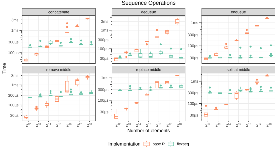
Figure 2: Benchmark timings for sequence operations.
