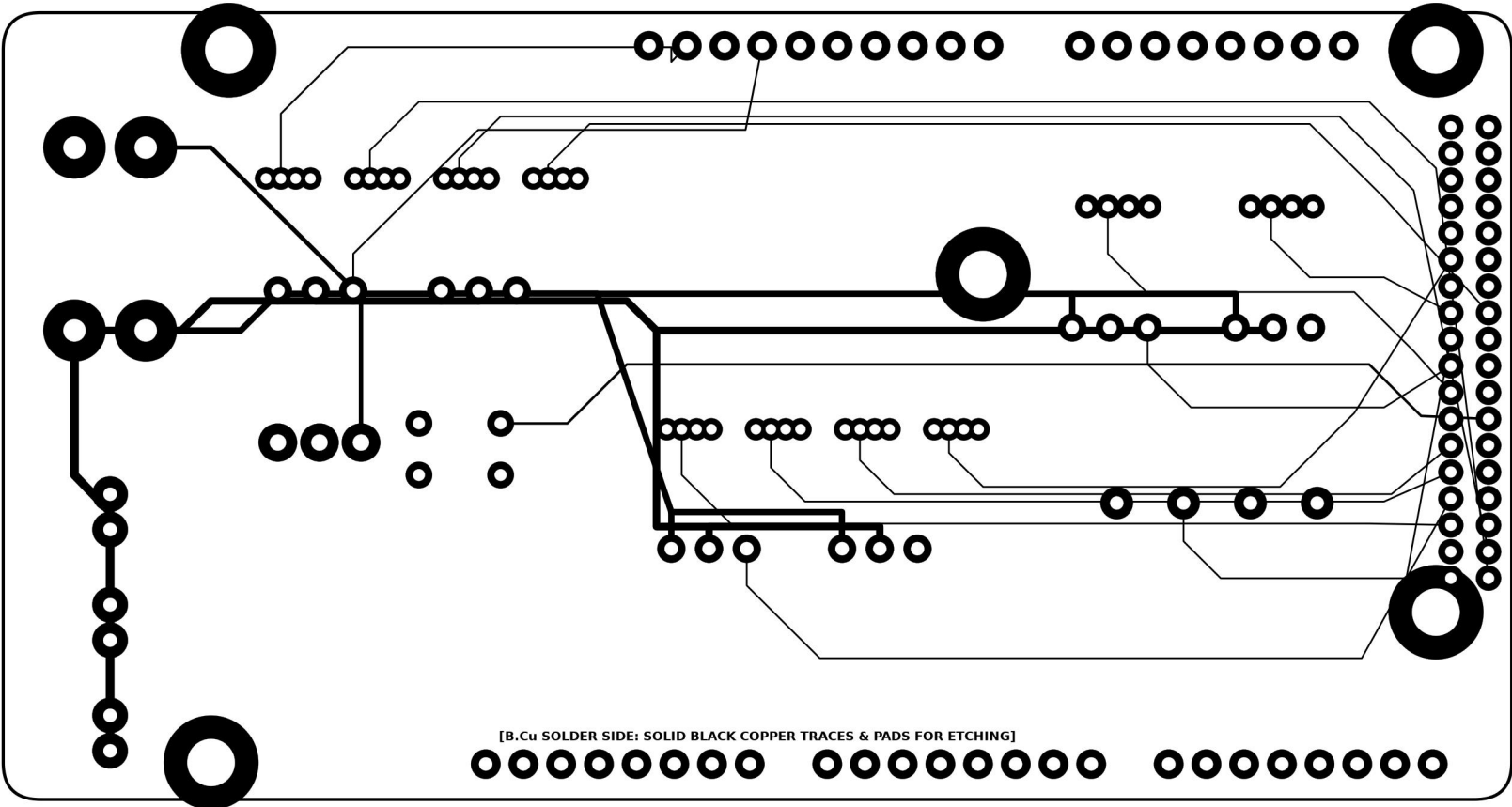
PANEL 1: BOTTOM COPPER ETCHING MASK (B.Cu - TONER TRANSFER / CNC MILLING)
