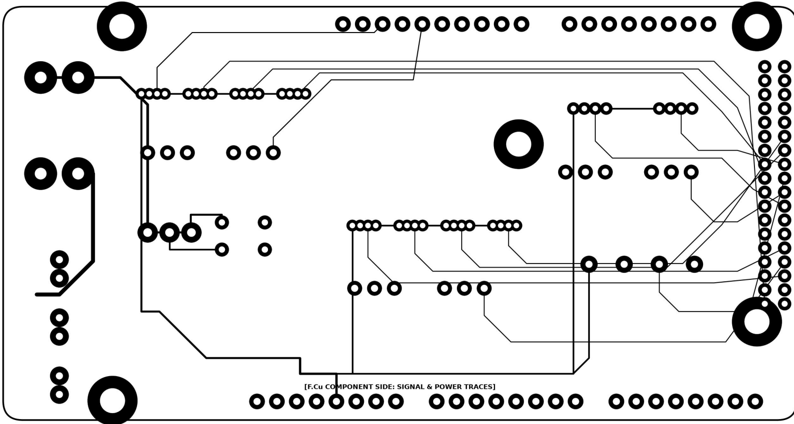
PANEL 2: TOP COPPER LAYER (F.Cu - COMPONENT SIDE TRACK ROUTING)
