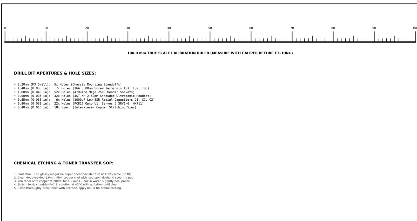
PANEL 4: 1:1 CALIBRATION RULER & DRILL BIT APERTURE SCHEDULE
