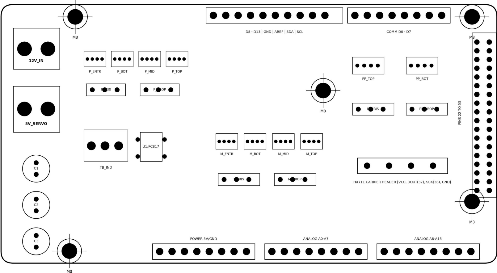
PANEL 3: TOP COMPONENT SILKSCREEN & DRILL POSITIONING TEMPLATE
