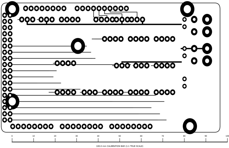
BOTTOM COPPER (B.Cu) — MIRRORED [IRON-ON / ETCH MASK]
