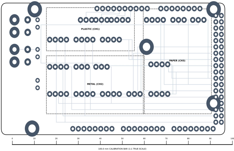
ASSEMBLY GUIDE & SILKSCREEN OVERLAY
