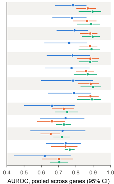
3–50 bp, without BRCA1
