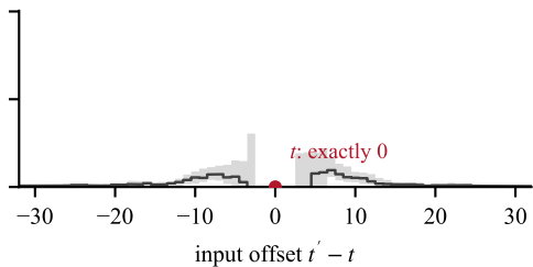
(b) evaluated patch masked
