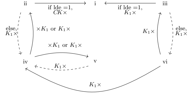
FIG. 1. Transitions between cases. The annotation K_1 \times ( \times K_1 ) on an arrow means that if A has the pattern at the tail, then K_1 \text{LAR} ( \text{LARK}_1 ) has the pattern at the head for suitably chosen generalized permutations L and R . Similarly for other annotations. Each of the dashed arrows preserves the \text{lde} , each of the rest decreases the \text{lde} by 1. Note that CK decomposes into a circuit with two K gates as in Equation (1).
