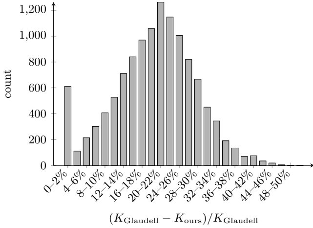
FIG. 3. Distribution of the relative K -count reduction (K_{\text{Glaudell}} - K_{\text{ours}})/K_{\text{Glaudell}} , binned in 2% increments. Our method improves on Glaudell et al.’s K -count in 95.1% of cases, with a mean reduction of 19.7%, a median of 20.3%, and a maximum of 50.0%.
