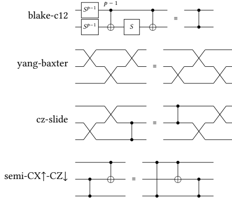
Fig. 2. The remaining two- and three-qubit rules. blake-c12 relates two circuits implementing controlled-Z; yang-baxter and cz-slide are the swap calculus.
