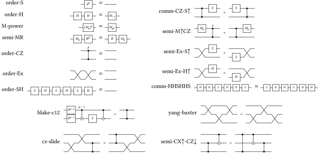
Fig. 1. The sixteen rules of \_CRel,=== as circuit equations. Diagrams read in matrix-multiplication order, so a word w \bullet v is drawn with v on the left. blake-c12 relates two circuits implementing controlled-Z; yang-baxter and cz-slide are the swap calculus.
