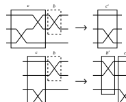
Fig. 3. Pushing a swap through a staircase: the four cases of the coset table \text{ract} as circuit rewrites.
