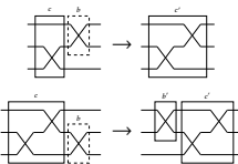
Fig. 3. Pushing a swap through a staircase: the four cases of the coset table \text{ract} as circuit rewrites.
