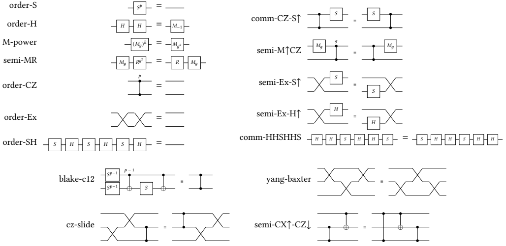
Fig. 2. The sixteen rules of _CRel,===_ as circuit equations. A word is drawn left to right as written and read in matrix-multiplication order, so in w \bullet v the right factor v acts first. blake-c12 relates two circuits implementing controlled-Z; yang-baxter and cz-slide are the swap calculus.
