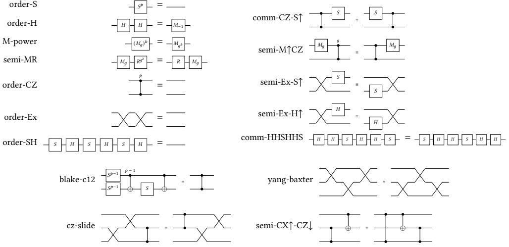
Fig. 2. The sixteen rules of _CRel_ as circuit equations. A word is drawn left to right as written and read in matrix-multiplication order, so in w \bullet v the right factor v acts first. blake-c12 relates two circuits implementing controlled- Z ; yang-baxter and cz-slide are the swap calculus.
