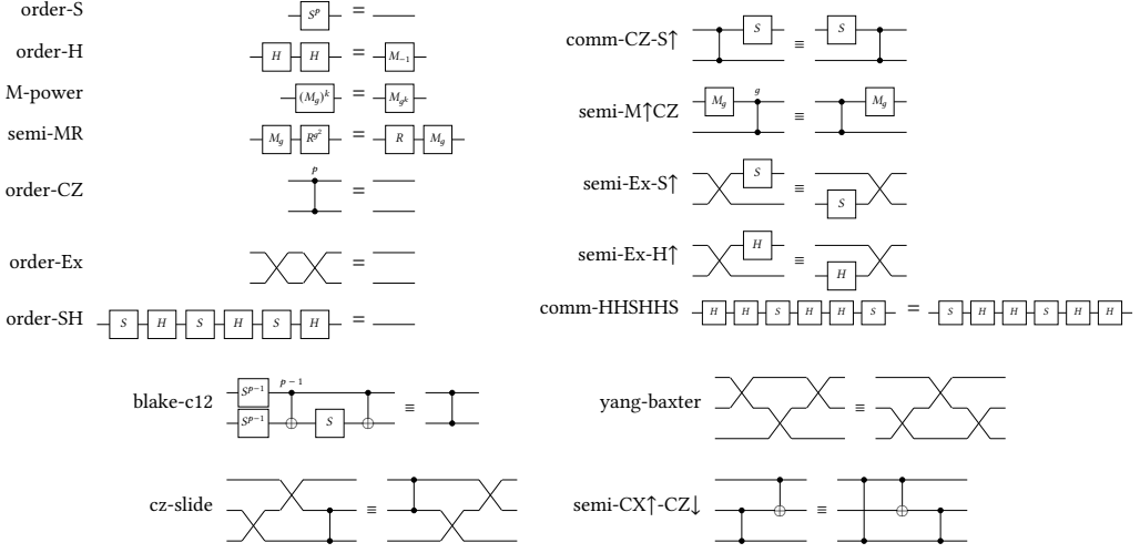
Fig. 3. The sixteen rules of Paper-V0's \_S\text{Rel}, \_==\_ as circuit equations. A word is drawn left to right as written and read in matrix-multiplication order, so in w \bullet v the right factor v acts first (§3.2). blake-c12 relates two circuits implementing controlled-Z; yang-baxter and cz-slide are the swap calculus.
