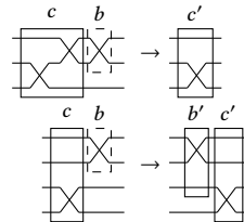
Fig. 4. Pushing a swap through a staircase: the four cases of the coset table ract as circuit rewrites.
