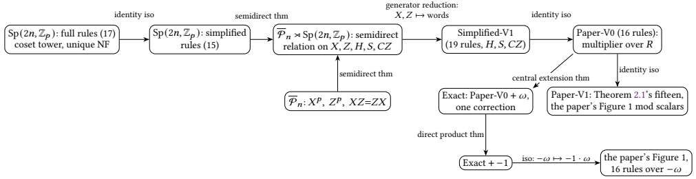
Fig. 2. The chain of presentations: every arrow is a verified presentation theorem or isomorphism of presentations; the semantic group is \text{Sp}(2n, \mathbb{Z}_p) on the left, \overline{\mathcal{P}}_n \rtimes \text{Sp}(2n, \mathbb{Z}_p) from the semidirect level on, a central extension of it by \langle \omega \rangle at “Exact”, and that times \langle -1 \rangle below it.
