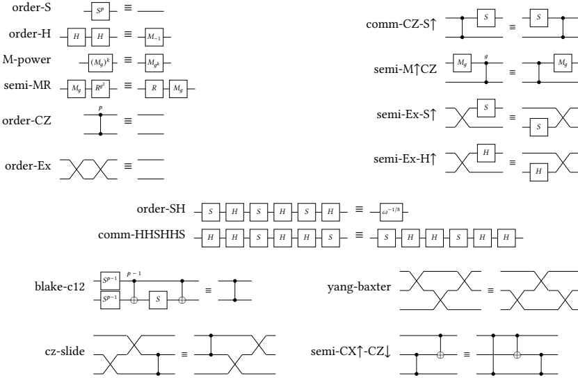
Fig. 3. The gate rules of the exact rule set _Exact, _===_ (§4) as circuit equations, drawn from the Agda terms: Paper-V0’s sixteen with the one correction, order-SH becoming (SH)^3 = \omega^{(p^2-1)/8} . Not drawn are the scalar’s own rules, \omega^p = \varepsilon and \omega commuting with every gate. Diagrams read in matrix-multiplication order (§2).
