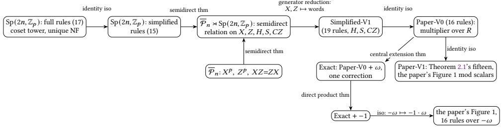
Fig. 2. The chain of presentations: every arrow is a verified presentation theorem or isomorphism of presentations; the semantic group is \text{Sp}(2n, \mathbb{Z}_p) on the left, \bar{\mathcal{P}}_n \rtimes \text{Sp}(2n, \mathbb{Z}_p) from the semidirect level on, a central extension of it by \langle \omega \rangle at “Exact”, and that times \langle -1 \rangle below it.
