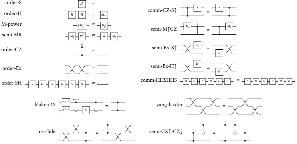
Fig. 3. The sixteen rules of Paper-V0's \_SRel,===\_ as circuit equations. A word is drawn left to right as written and read in matrix-multiplication order, so in w \bullet v the right factor v acts first (§3.2). blake-c12 relates two circuits implementing controlled-Z; yang-baxter and cz-slide are the swap calculus.
