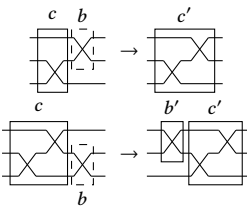
Fig. 1. Pushing a swap through a staircase: the four cases of the coset table ract as circuit rewrites.
