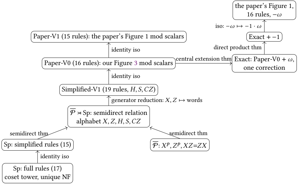
Fig. 2. The chain of presentations. Every arrow is a verified presentation theorem or a verified isomorphism of presentations; the semantic group is \text{Sp}(2n, \mathbb{Z}_p) at the bottom, \bar{\mathcal{P}}_n \rtimes \text{Sp}(2n, \mathbb{Z}_p) from the semidirect level up, a central extension of it by \langle \omega \rangle at the right, and that times \langle -1 \rangle above it.
