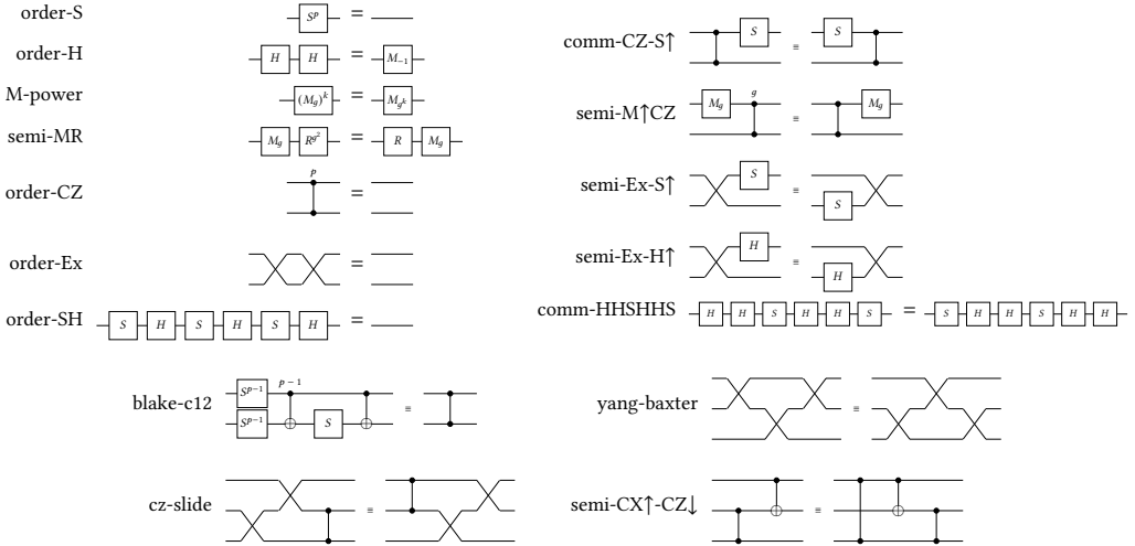
Fig. 1. The sixteen rules of _CRel_ (§2) as circuit equations, drawn from the Agda terms. Diagrams read in matrix-multiplication order, so a word w \bullet v is drawn with v on the left. blake-c12 relates two circuits implementing controlled-Z; yang-baxter and cz-slide are the swap calculus. With the scalar restored (§5) only order-SH changes, to (SH)^3 = \omega^{-1/8} .
