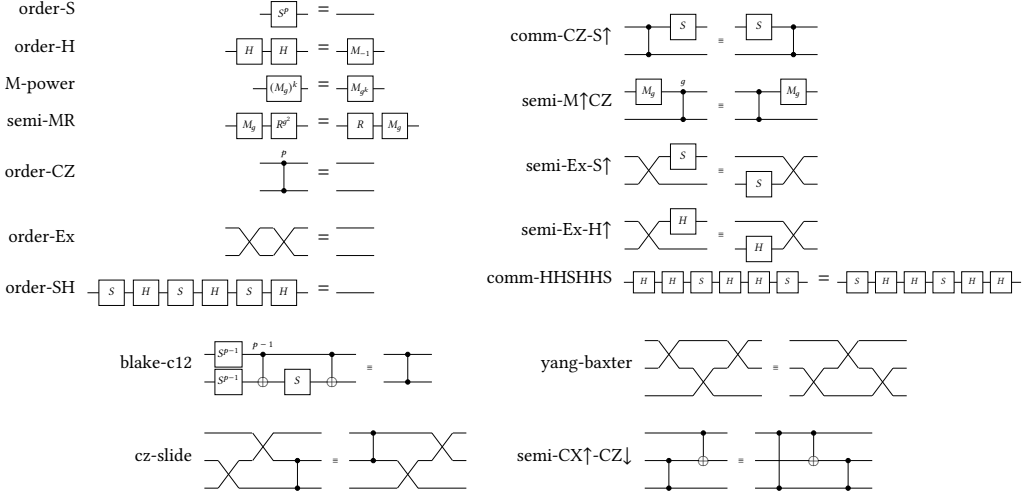
Fig. 3. The sixteen rules of \_CRel\_ as circuit equations. A word is drawn left to right as written and read in matrix-multiplication order, so in w \bullet v the right factor v acts first. blake-c12 relates two circuits implementing controlled-Z; yang-baxter and cz-slide are the swap calculus.
