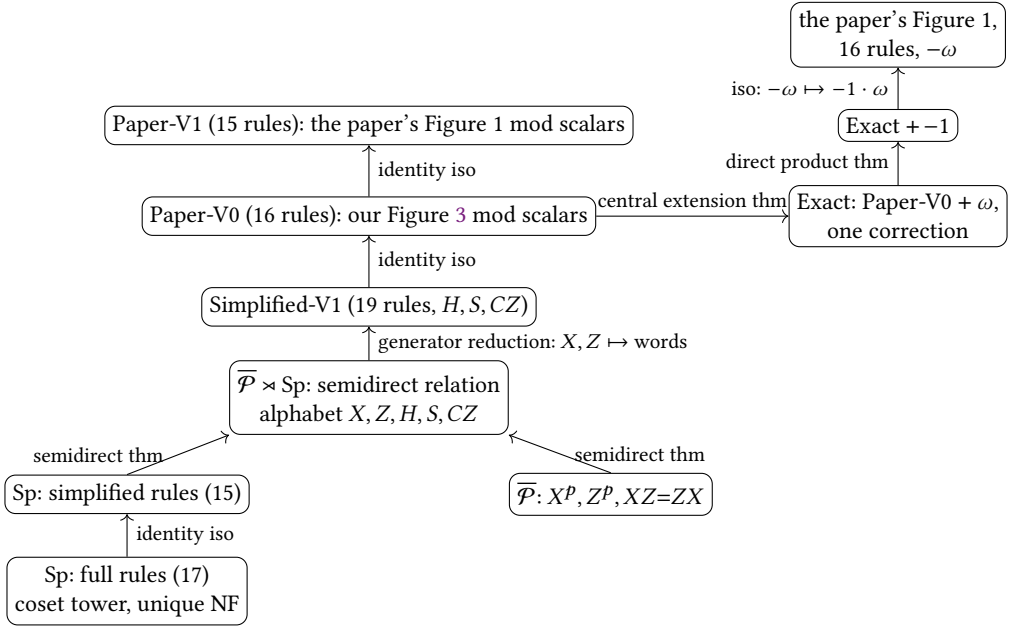
Fig. 2. The chain of presentations. Every arrow is a verified presentation theorem or a verified isomorphism of presentations; the semantic group is \text{Sp}(2n, \mathbb{Z}_p) at the bottom, \overline{\mathcal{P}}_n \rtimes \text{Sp}(2n, \mathbb{Z}_p) from the semidirect level up, a central extension of it by \langle \omega \rangle at the right, and that times \langle -1 \rangle above it.
