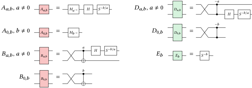
Fig. 2. The four kinds of normal box (the qupit paper’s Figure 6) and how each is spelled as a circuit by the section of the normal form (§5).
