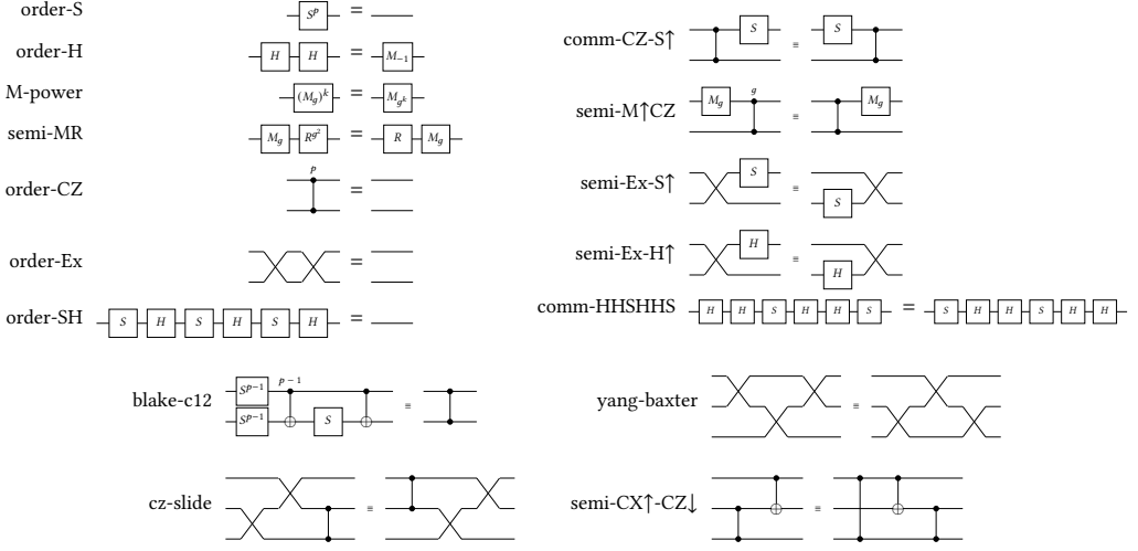
Fig. 2. The sixteen rules of \text{CRel}_{===} as circuit equations. A word is drawn left to right as written and read in matrix-multiplication order, so in w \bullet v the right factor v acts first. blake-c12 relates two circuits implementing controlled-Z; yang-baxter and cz-slide are the swap calculus.
