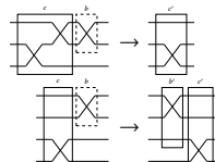
Fig. 1. Pushing a swap through a staircase: the four cases of the coset table ract as circuit rewrites.
