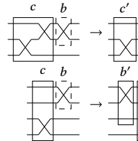
Fig. 1. Pushing a swap through a staircase: the four cases of the coset table ract as circuit rewrites.
