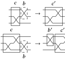
Fig. 1. Pushing a swap through a staircase: the four cases of the coset table ract as circuit rewrites.
