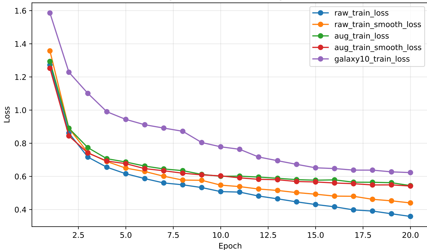
Training Loss (raw, smooth, augmented)
