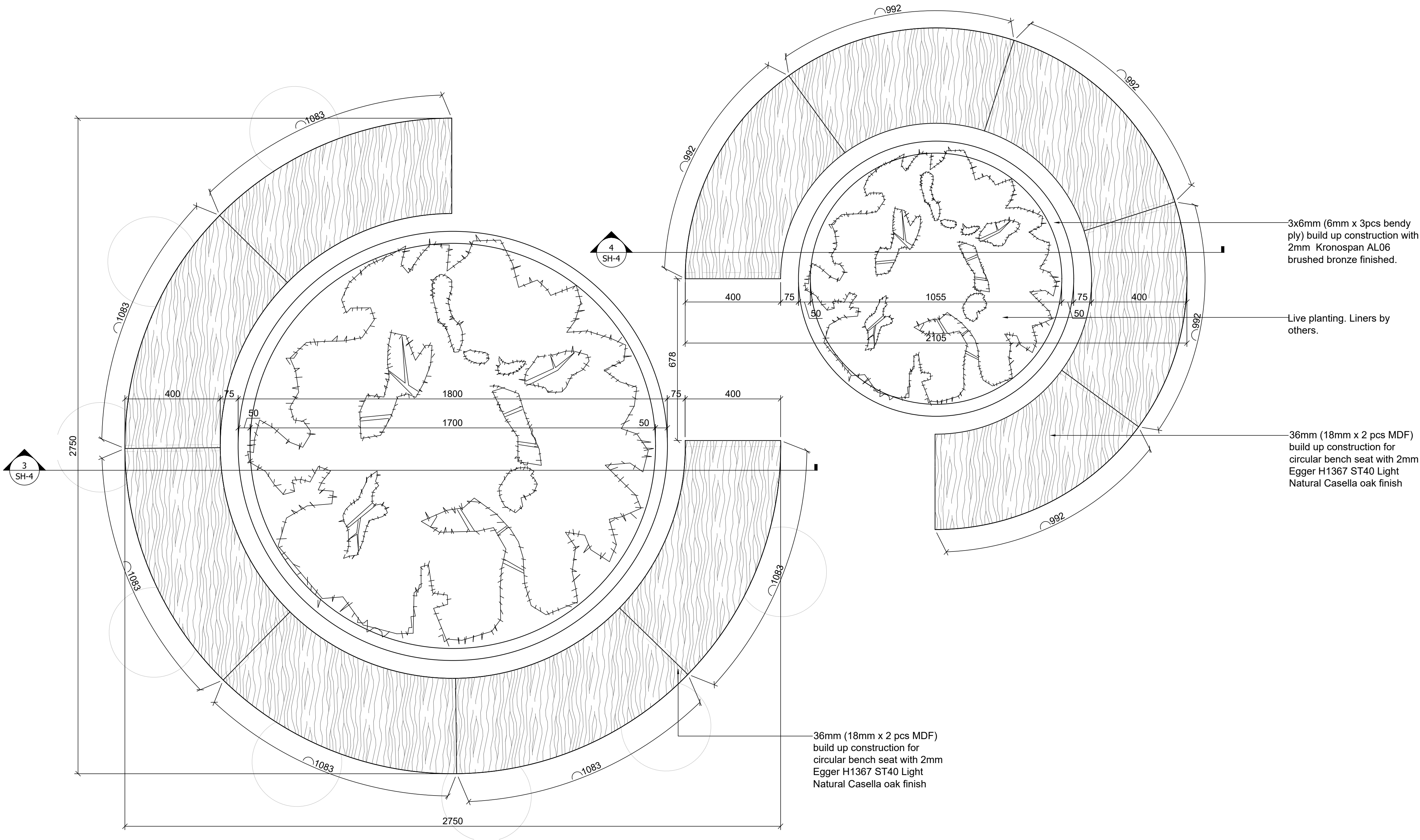
1 PLAN
