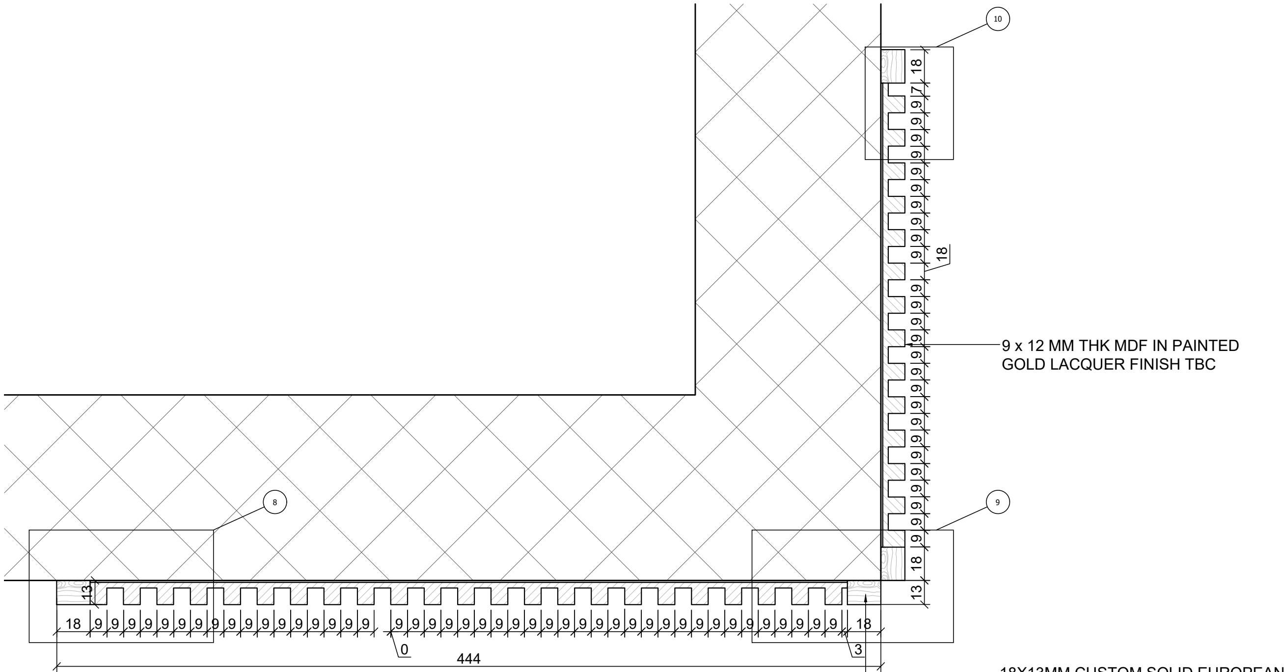
6 PLAN DETAILS Scale: 1:2
