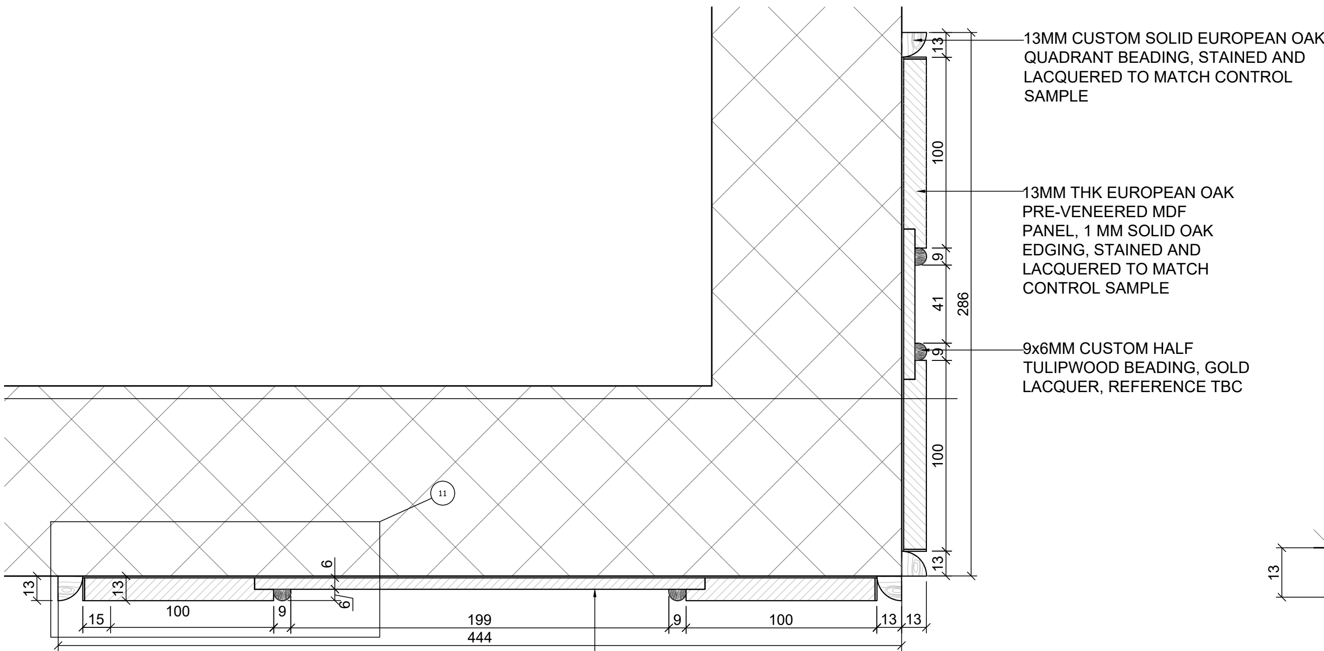
7 PLAN DETAILS Scale: 1:2
