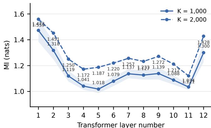
MusicBERT LMD-matched: Duration
