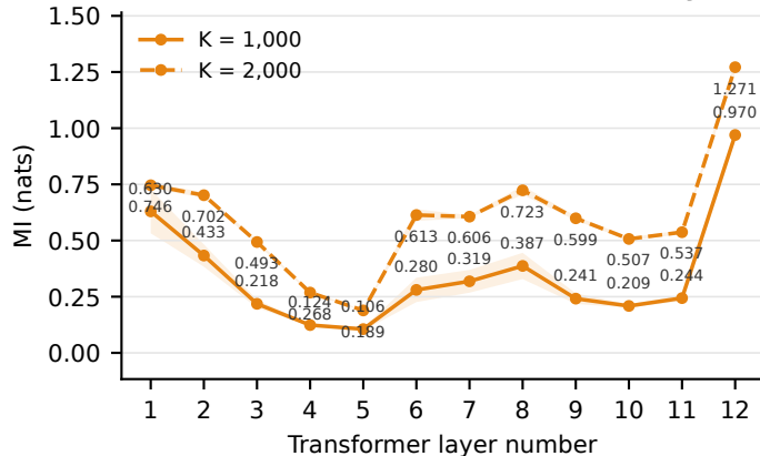
MusicBERT LMD-matched: Tempo
