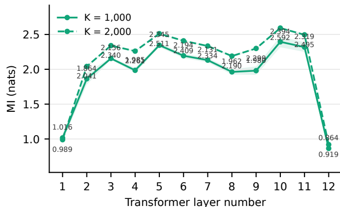
MusicBERT LMD-matched: Pitch
