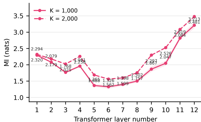
MusicBERT LMD-matched: Velocity
