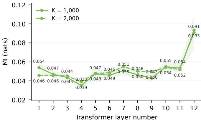
MusicBERT LMD-matched: Time signature
