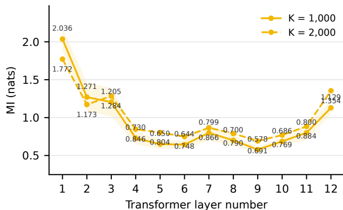
MusicBERT LMD-matched: Time signature
