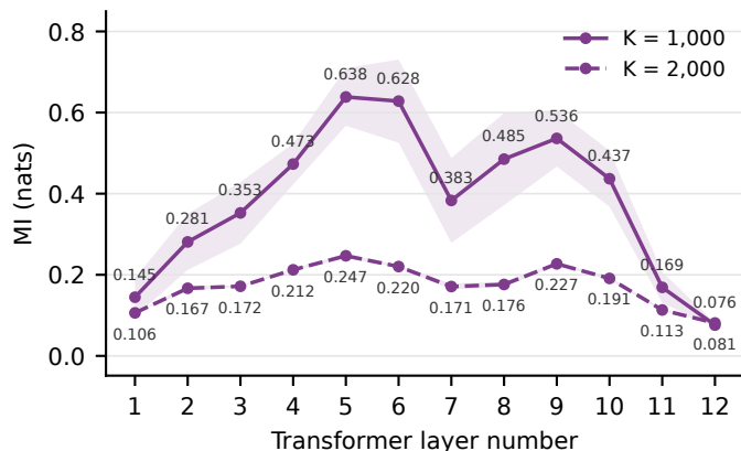
MusicBERT LMD-matched: Instrument
