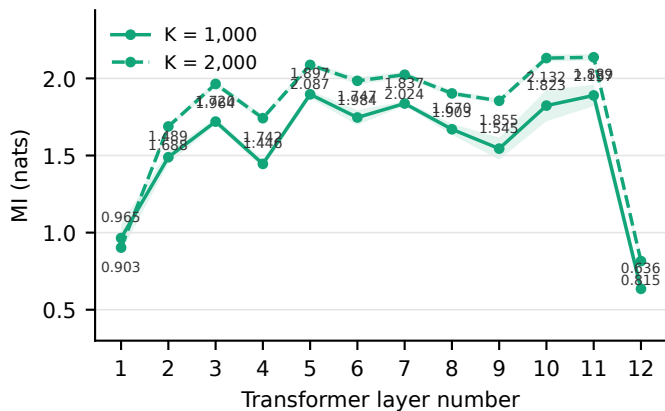
MusicBERT SOD: Pitch
