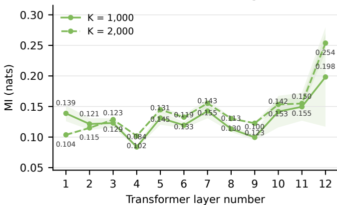
MusicBERT SOD: Time signature
