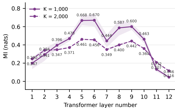
MusicBERT SOD: Instrument
