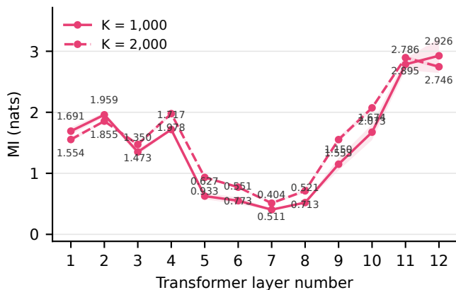
MusicBERT SOD: Velocity
