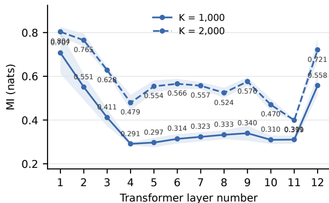
MusicBERT SOD: Duration
