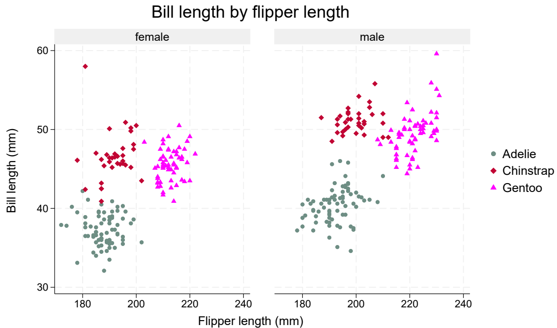
Figure 3: Penguin measurements by sex and species. Source: Horst, Hill, and Gorman (2020).
