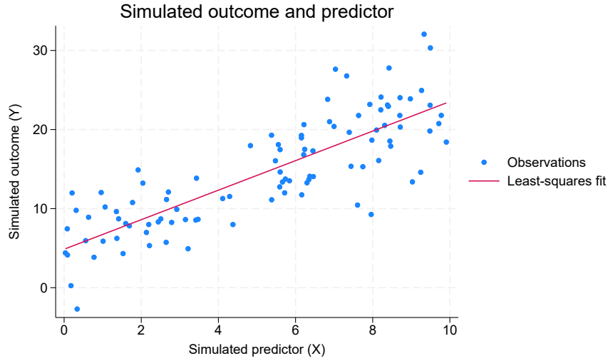
Figure 1: Simulated outcome (Y) and predictor (X), with a least-squares fit.
