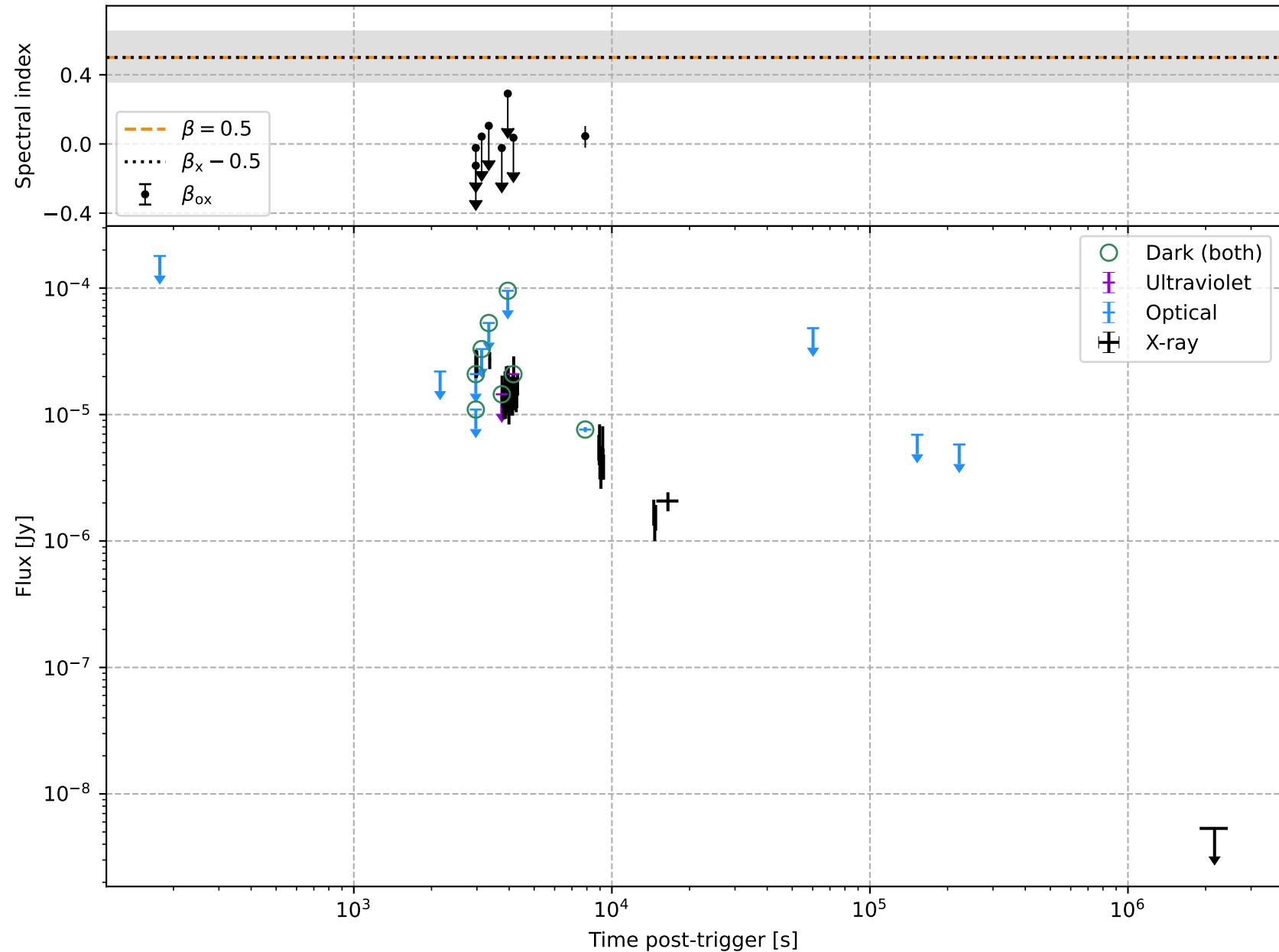
GRB 201216C: 8 dark points
