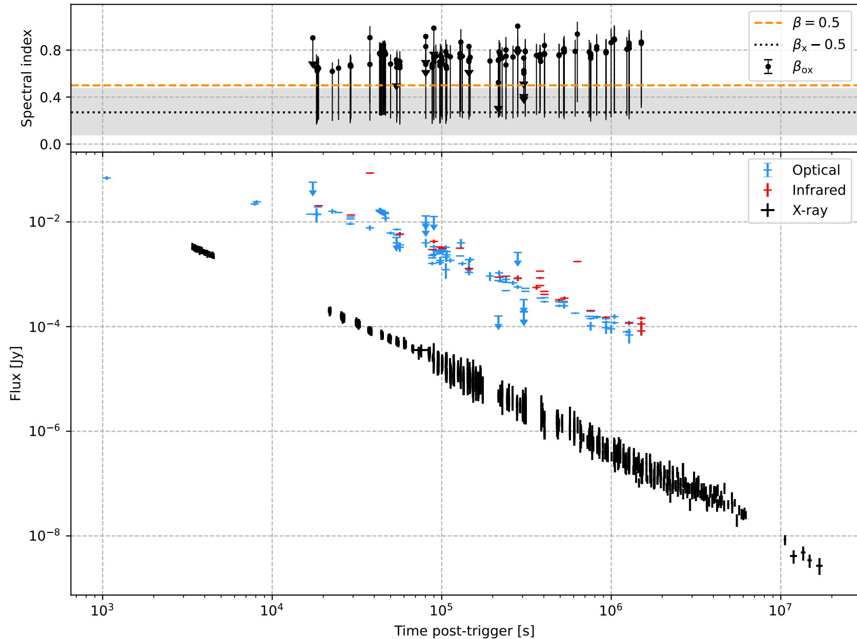
GRB 221009A: 0 dark points
