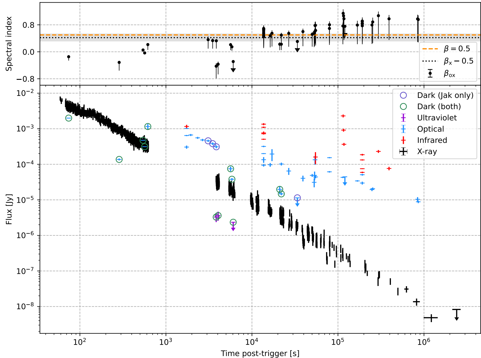
GRB 190114C: 16 dark points
