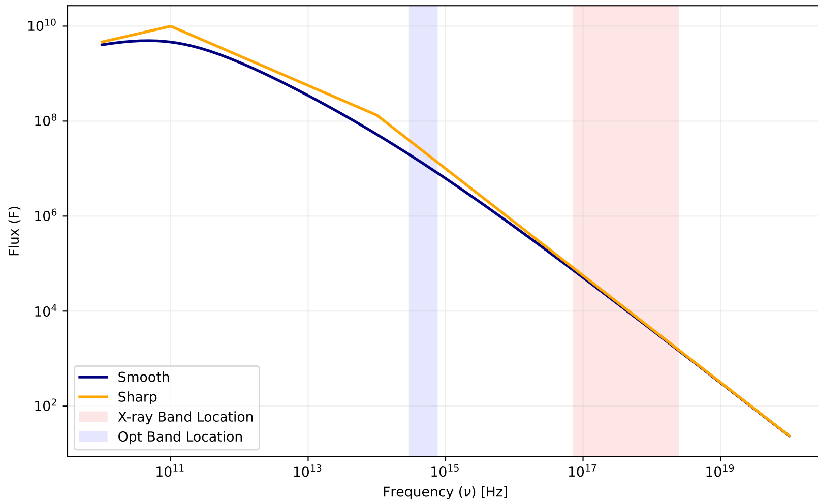
Smooth vs. Sharp Spectral Model ( p = 2.25 , \nu_c = 1.000\text{e}+14 )
