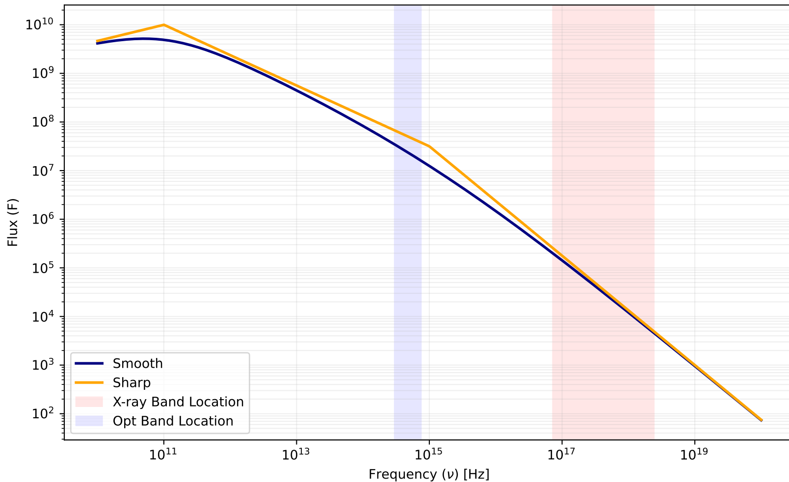
Smooth vs. Sharp Spectral Model ( p = 2.25 , \nu_c = 1.000\text{e}+15 )
