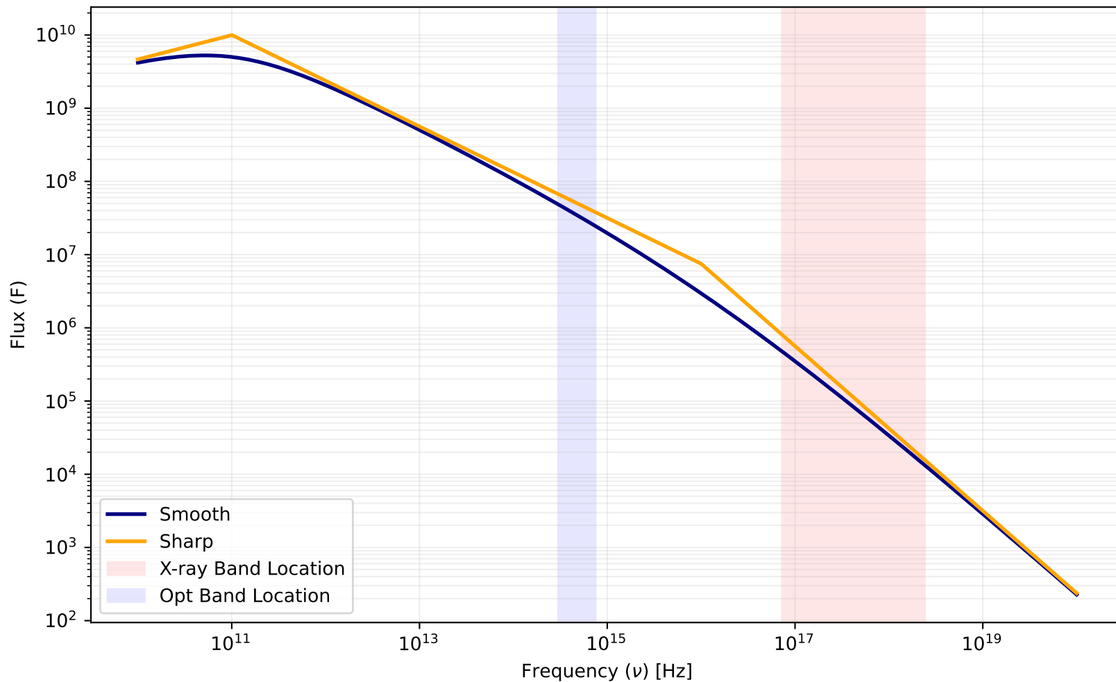
Smooth vs. Sharp Spectral Model ( p = 2.25 , \nu_c = 1.000\text{e}+16 )
