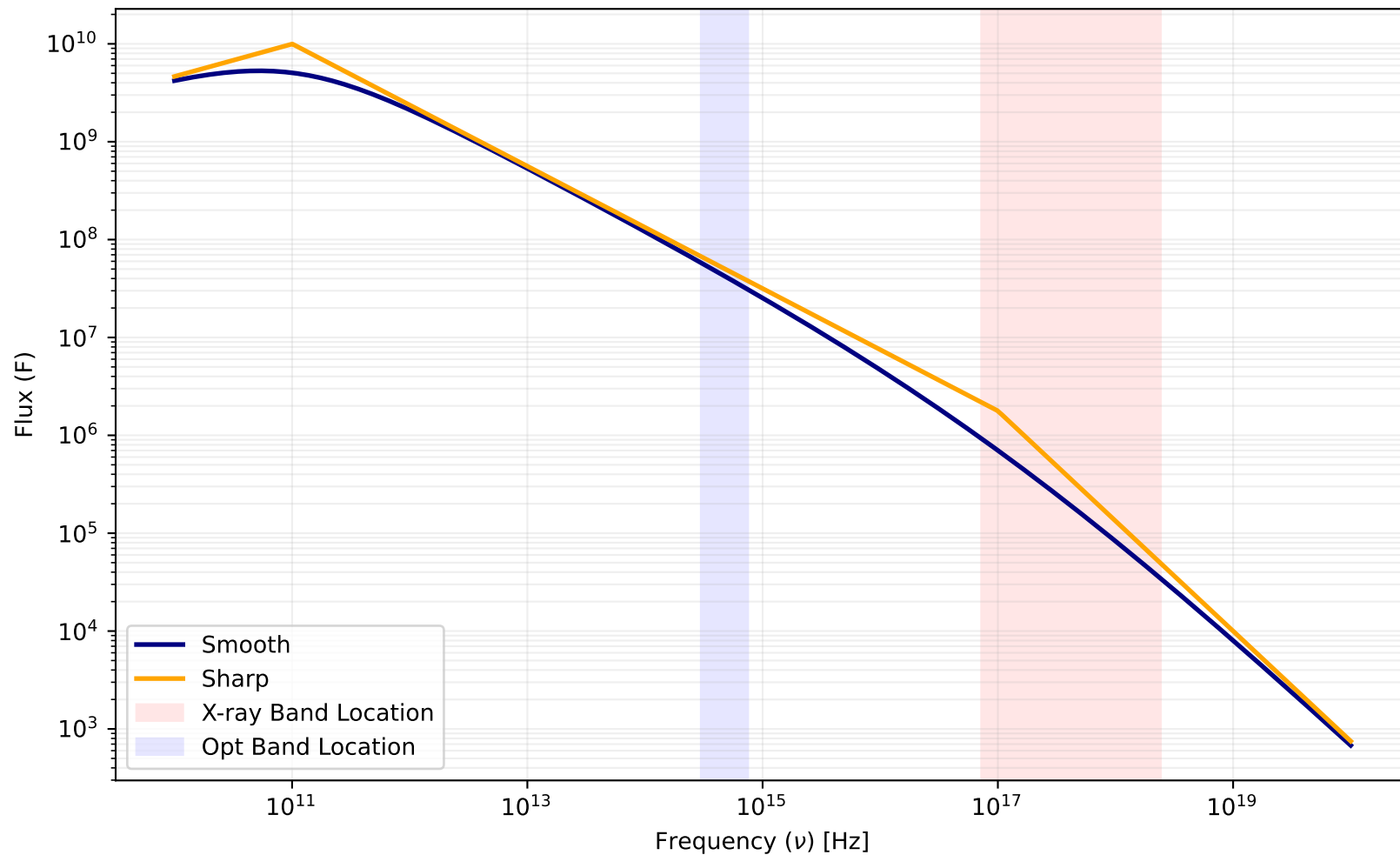
Smooth vs. Sharp Spectral Model ( p = 2.25 , \nu_c = 1.000\text{e}+17 )
