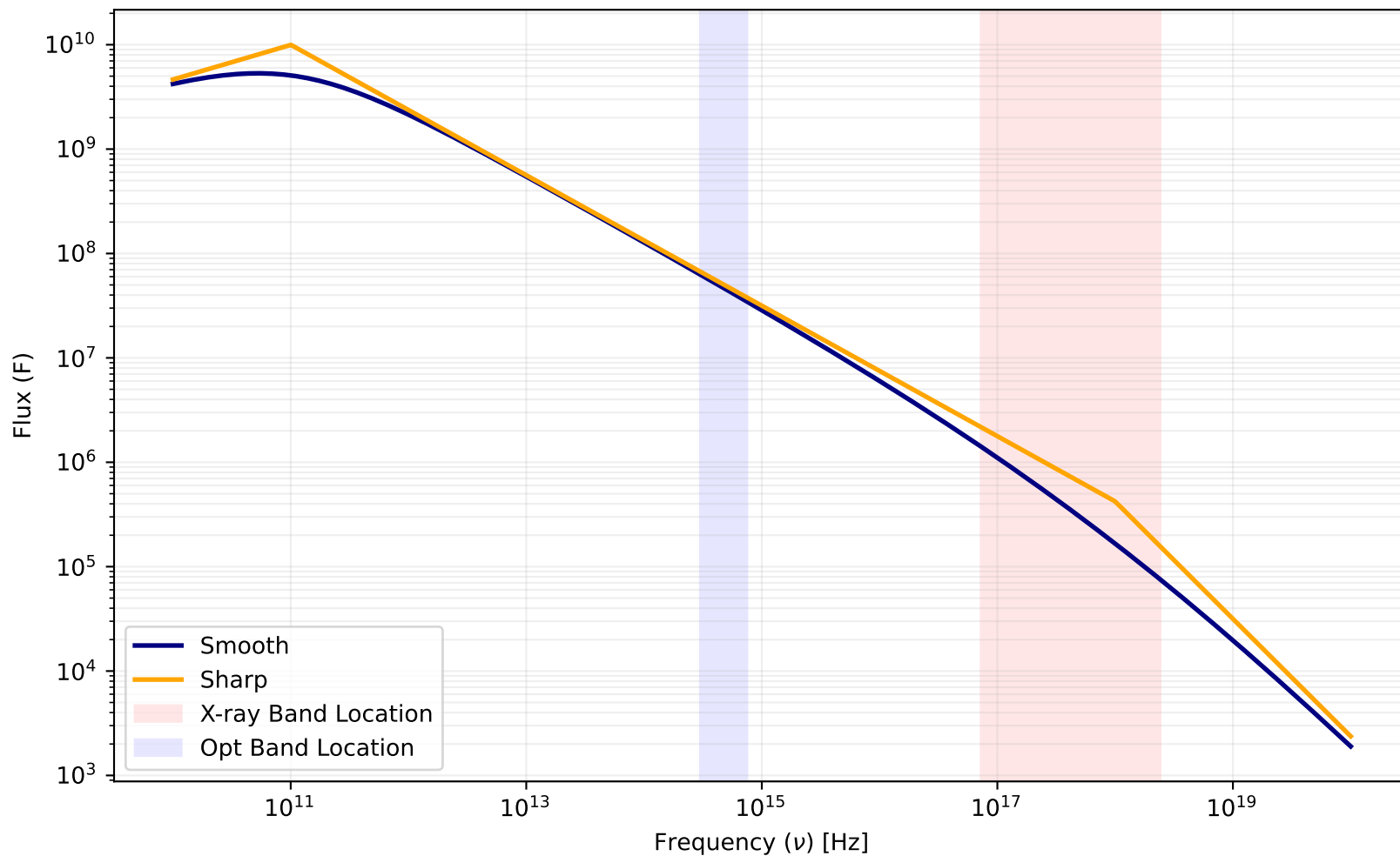
Smooth vs. Sharp Spectral Model ( p = 2.25 , \nu_c = 1.000\text{e}+18 )
