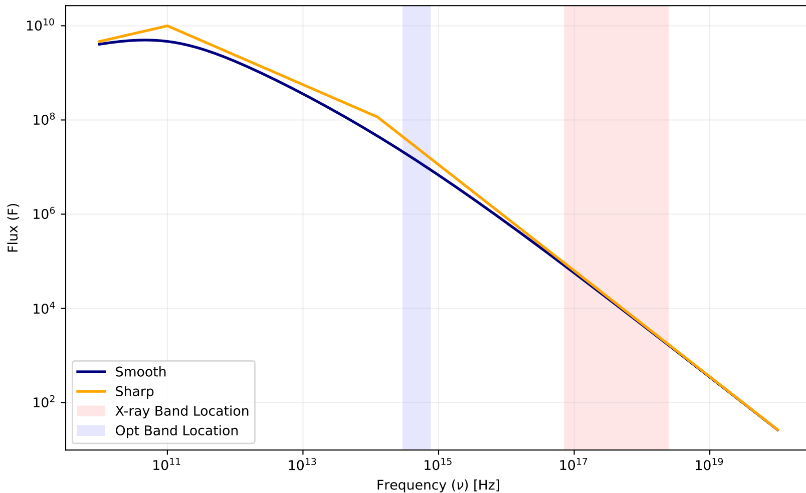
Smooth vs. Sharp Spectral Model ( p = 2.25 , \nu_c = 1.259\text{e}+14 )
