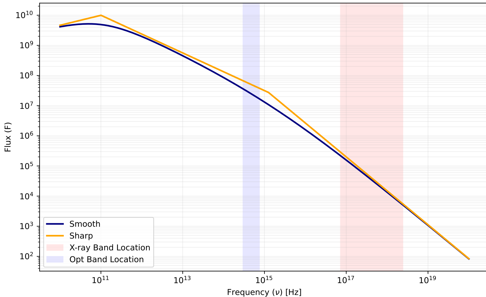
Smooth vs. Sharp Spectral Model ( p = 2.25 , \nu_c = 1.259\text{e}+15 )
