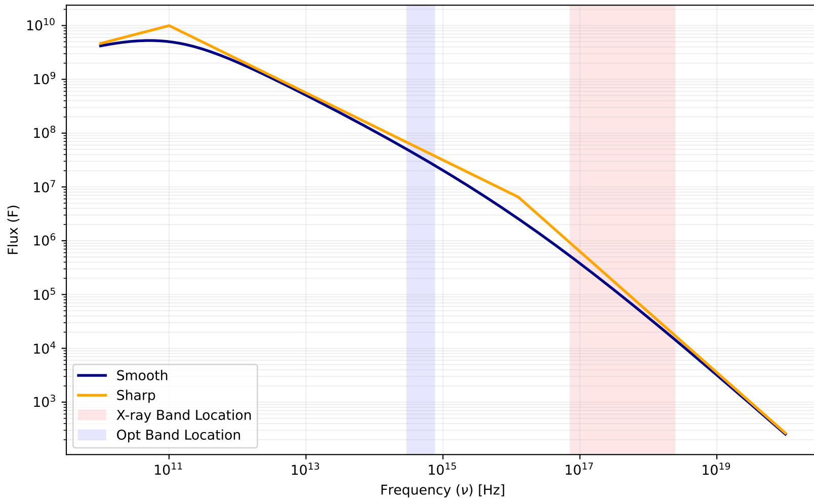
Smooth vs. Sharp Spectral Model ( p = 2.25 , \nu_c = 1.259\text{e}+16 )
