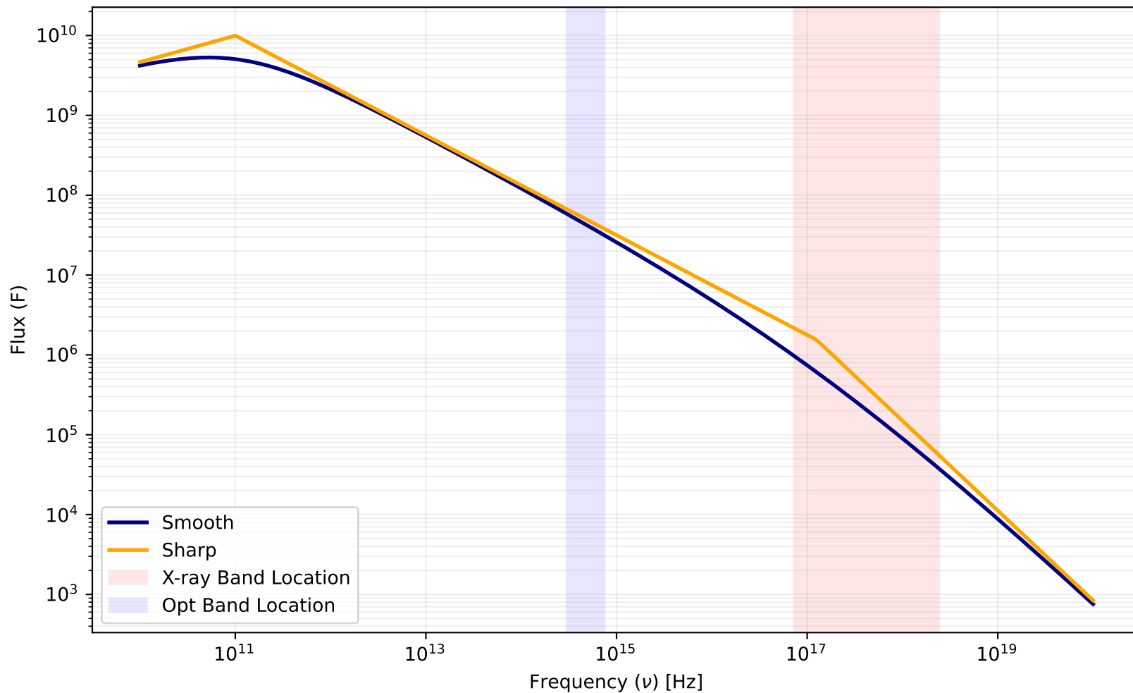
Smooth vs. Sharp Spectral Model ( p = 2.25 , \nu_c = 1.259\text{e}+17 )
