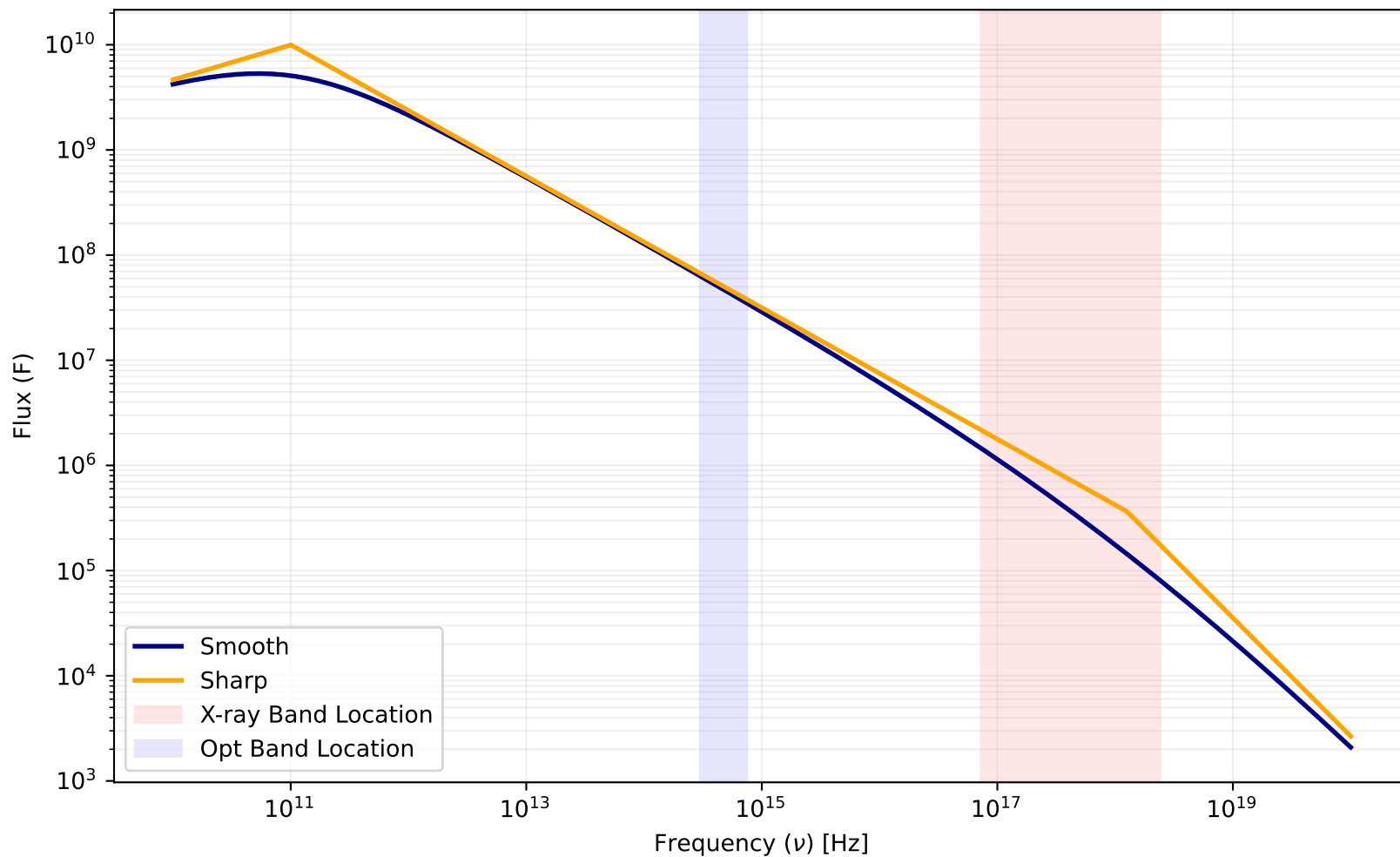
Smooth vs. Sharp Spectral Model ( p = 2.25 , \nu_c = 1.259\text{e}+18 )
