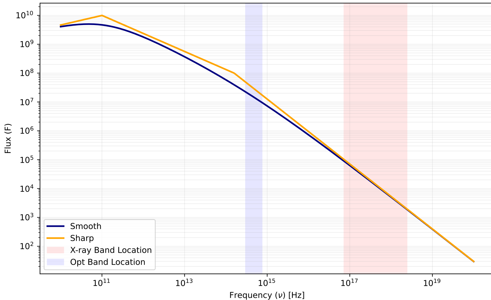
Smooth vs. Sharp Spectral Model ( p = 2.25 , \nu_c = 1.585\text{e}+14 )
